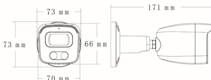
Dimensions (mm)
