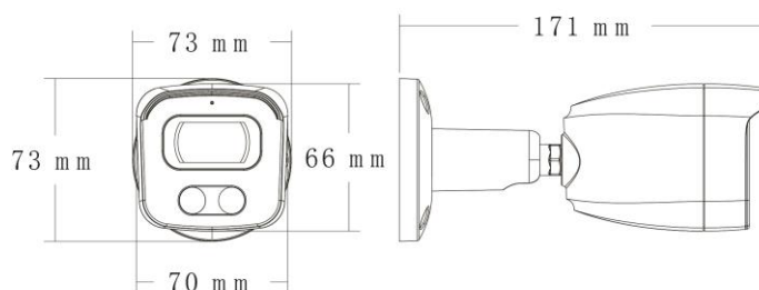
Dimensions (mm)
